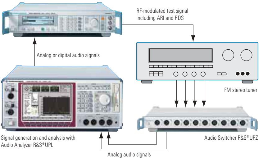
The Audio Switcher R&S®UPZ for automated measurements on more than two audio outputs.
