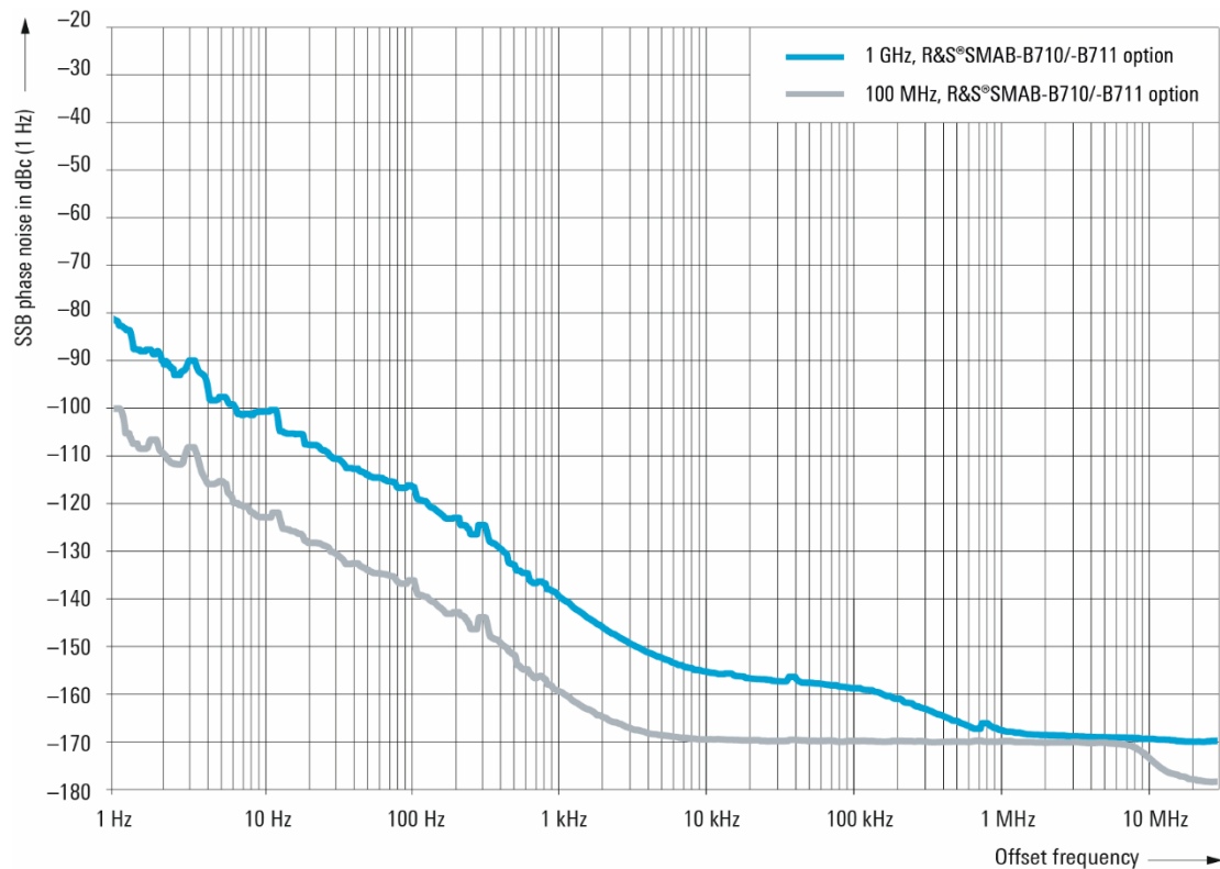
Measured SSB phase noise of reference outputs at f = 100 MHz and 1 GHz with the R&S®SMAB-B710(N) and R&S®SMAB-B711(N) options (only available with the R&S®SMAB-K703 option).
