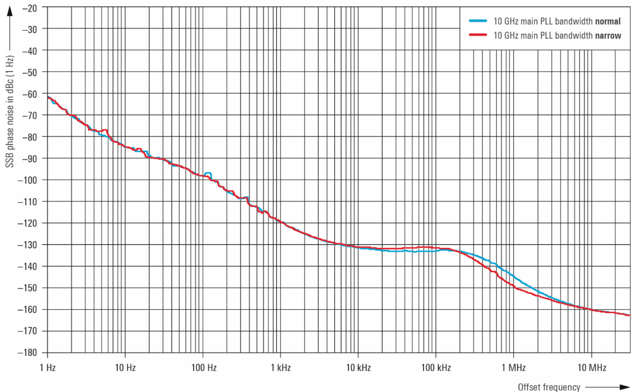
Measured SSB phase noise at f = 10 GHz, comparison of PLL bandwidth normal and narrow with the R&S®SMAB-B711 option.
