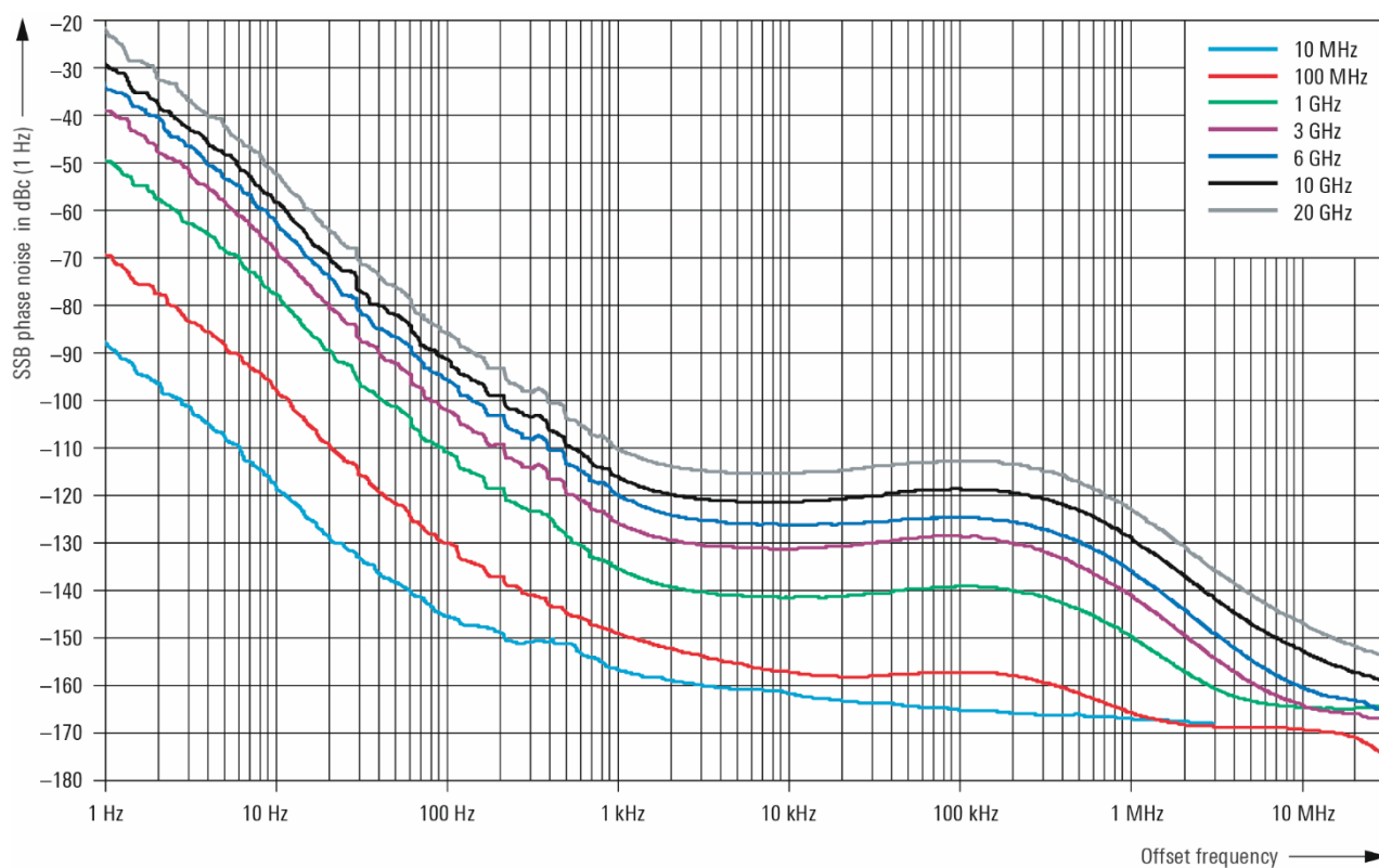
Measured SSB phase noise (standard performance).
