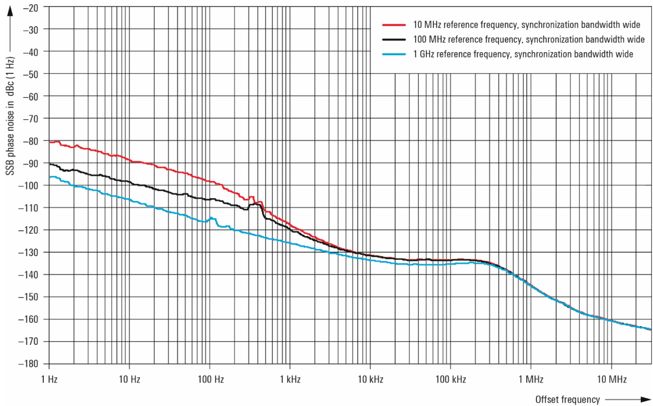
Measured residual SSB phase noise at f = 10 GHz with the R&S®SMAB-B711 option, comparison of different reference frequencies.
