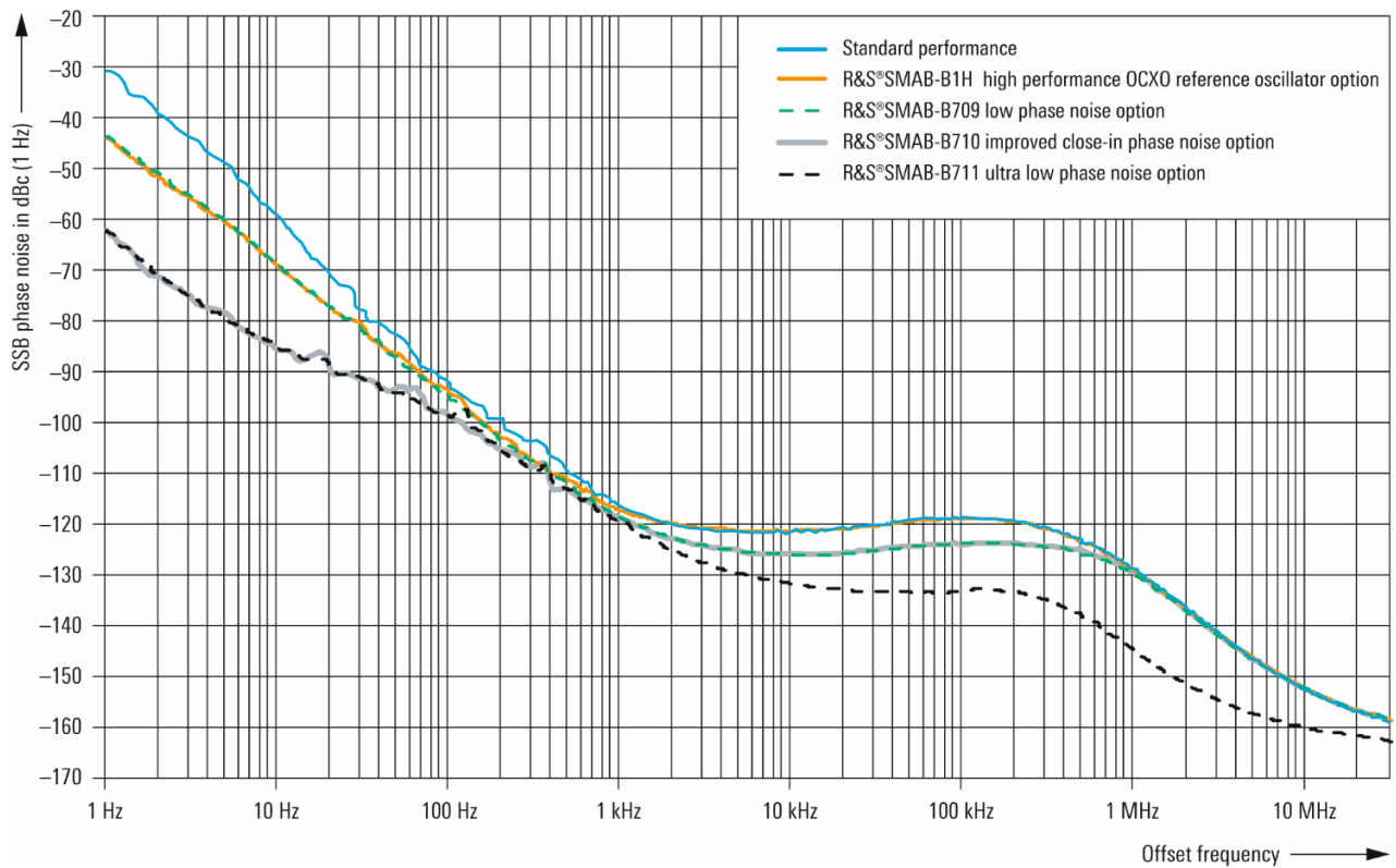
Measured SSB phase noise at f = 10 GHz, standard performance versus the R&S®SMAB-B1H, R&S®SMAB-B709, R&S®SMAB-B710 and R&S®SMAB-B711 options.
