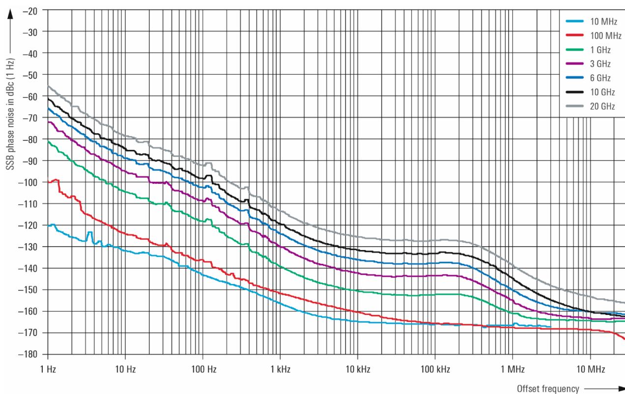
Measured SSB phase noise with the R&S®SMAB-B711(N) option.
