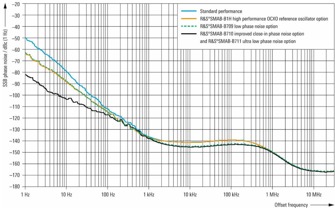
Measured SSB phase noise of clock synthesizer at f = 1 GHz, standard performance versus the R&S®SMAB-B1H, R&S®SMAB-B709, R&S®SMAB-B710(N) and R&S®SMAB-B711(N) options.
