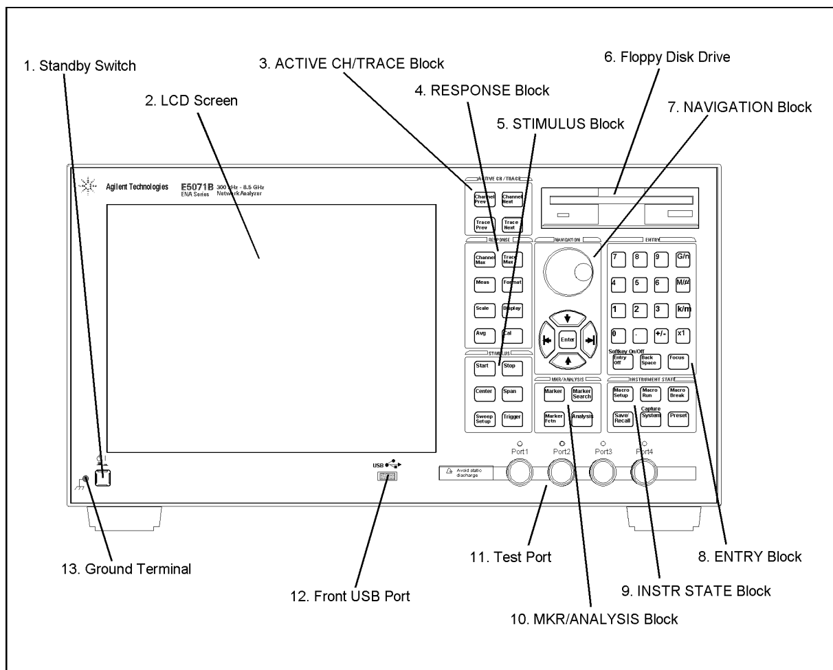
Figure 3-1 Front Panel
